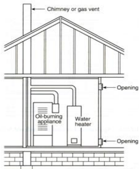
FIGURE 703.2.1 Appliances Located in Confined Spaces – All Air Taken from Inside the Building
