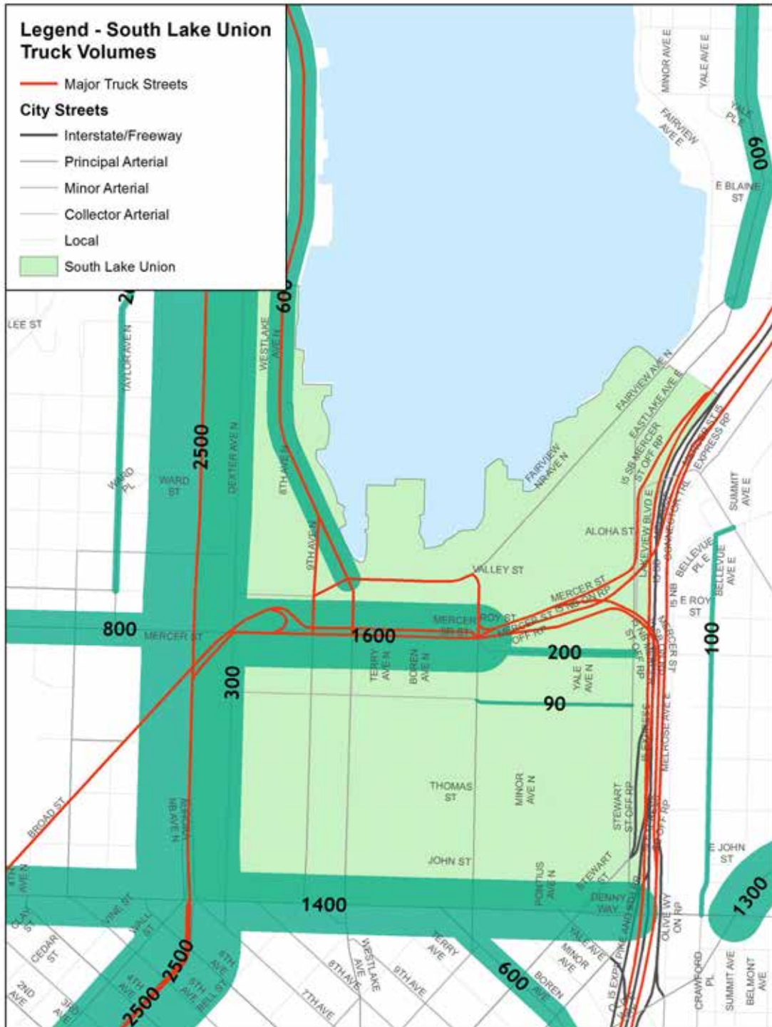
Figure 14: South Lake Union Daily Truck Volumes. Source: SDOT GIS FreightFlow_segments_final layer, 2015
