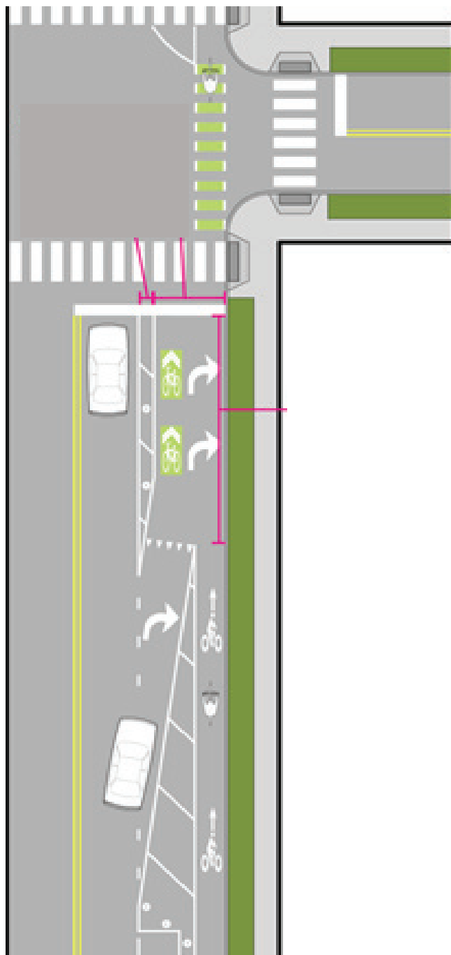
Figure 4: One-way Protected Bicycle Lane Mixing Zone
