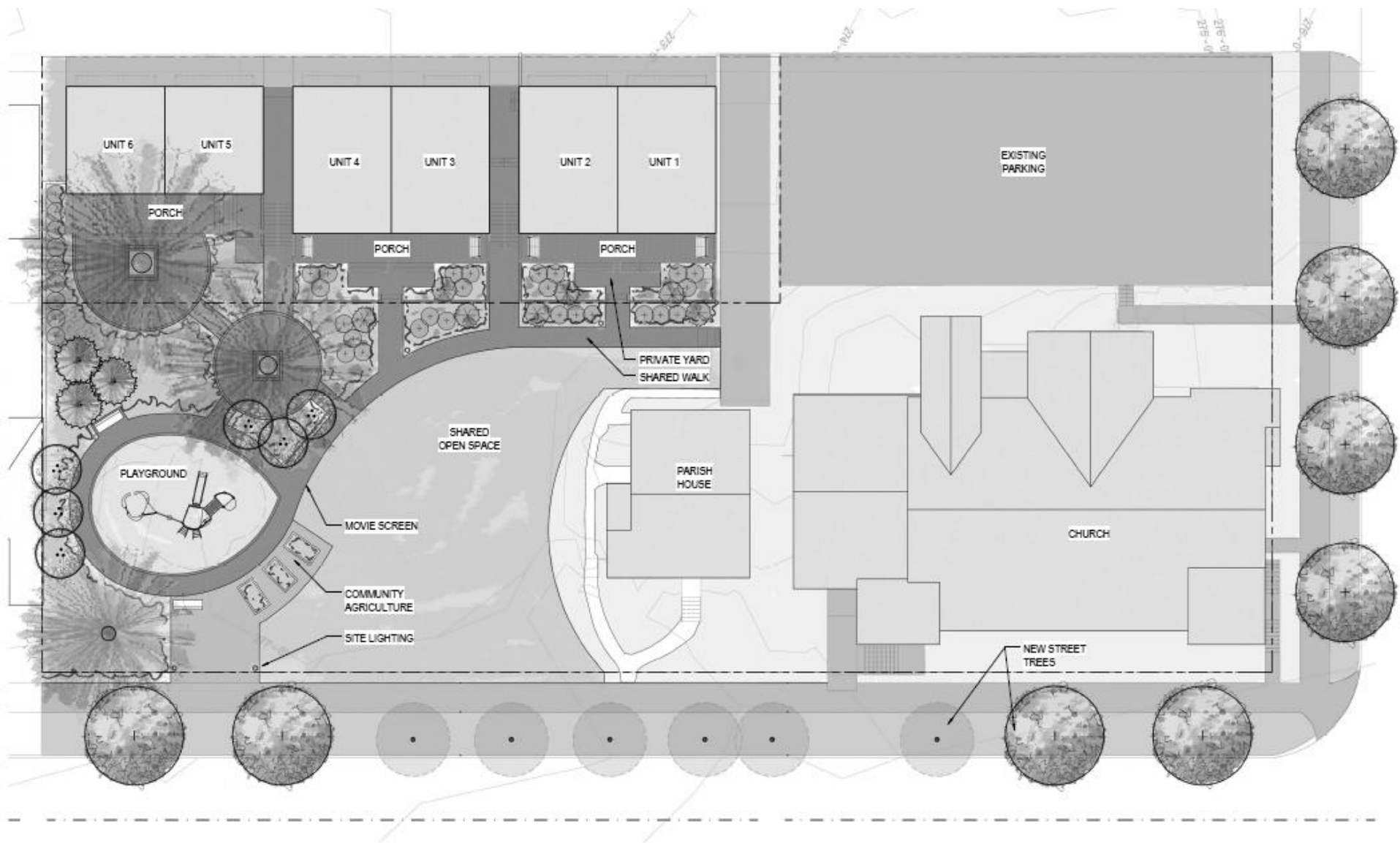
Detail from HE Exhibit 11, Landscape Plan, Sheet L1
