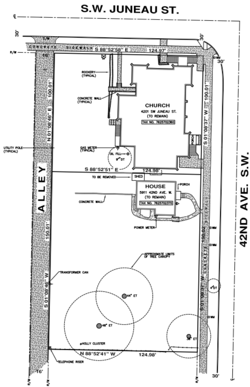
EXISTING SITE CONDITIONS DETAIL
