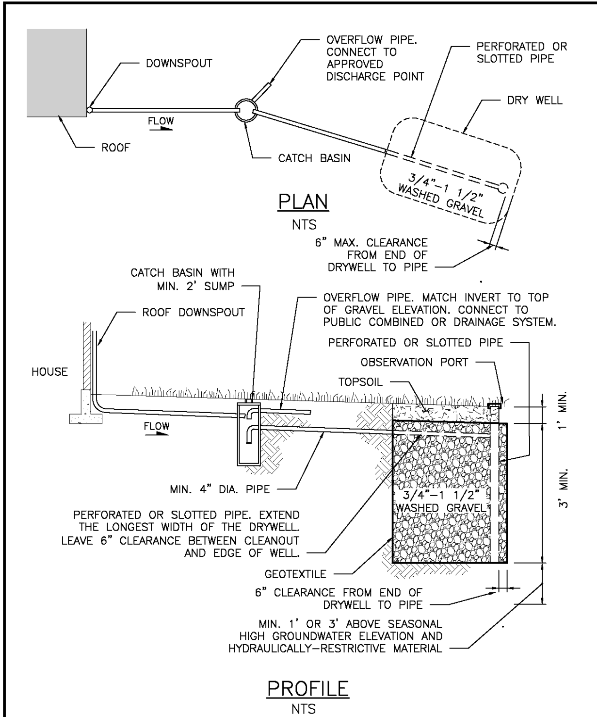
Figure 5.105-9. Typical Infiltration Drywell.
