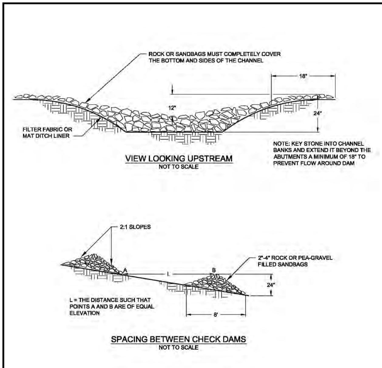
Figure 9. Check Dams.
