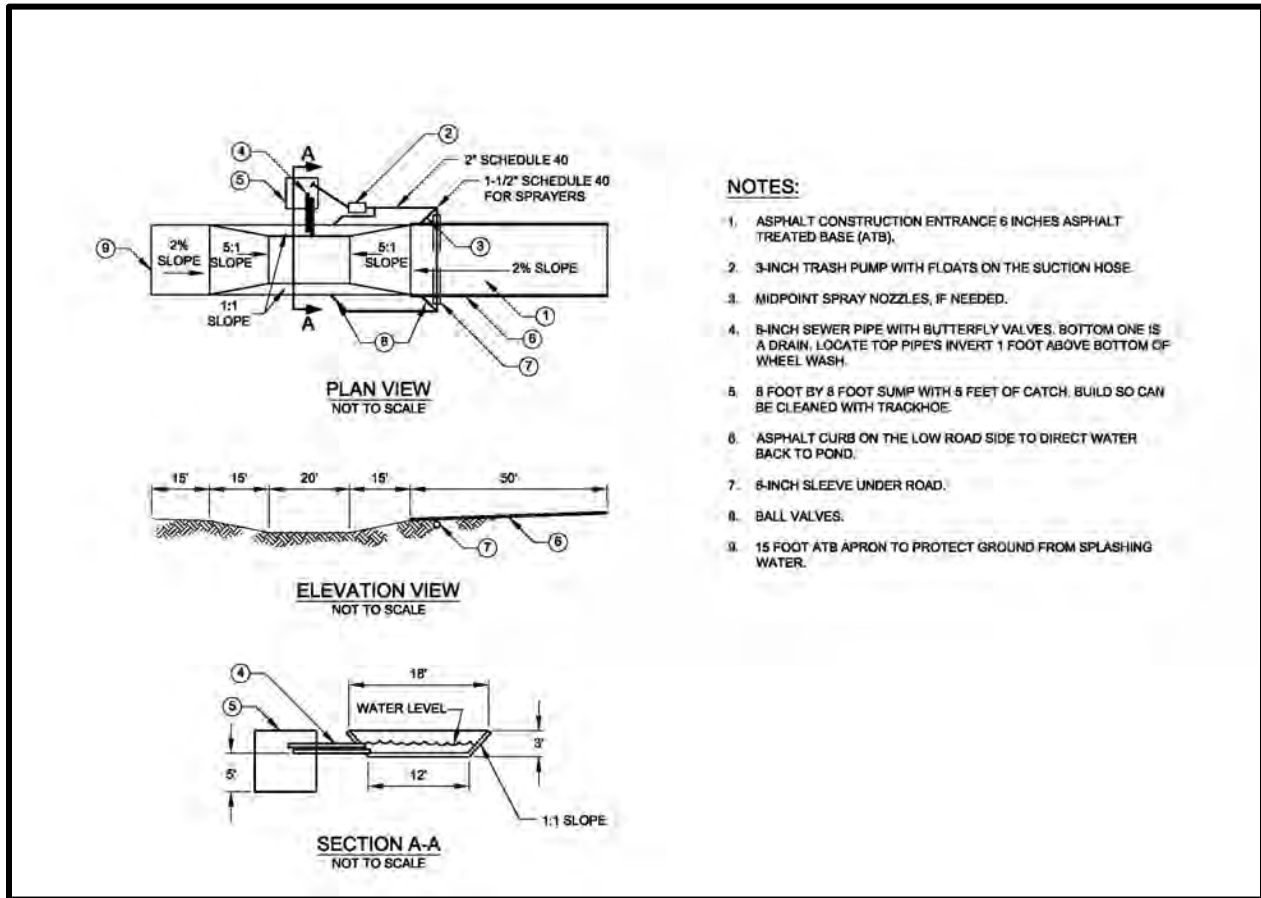
Figure 8. Tire Wash Details.
