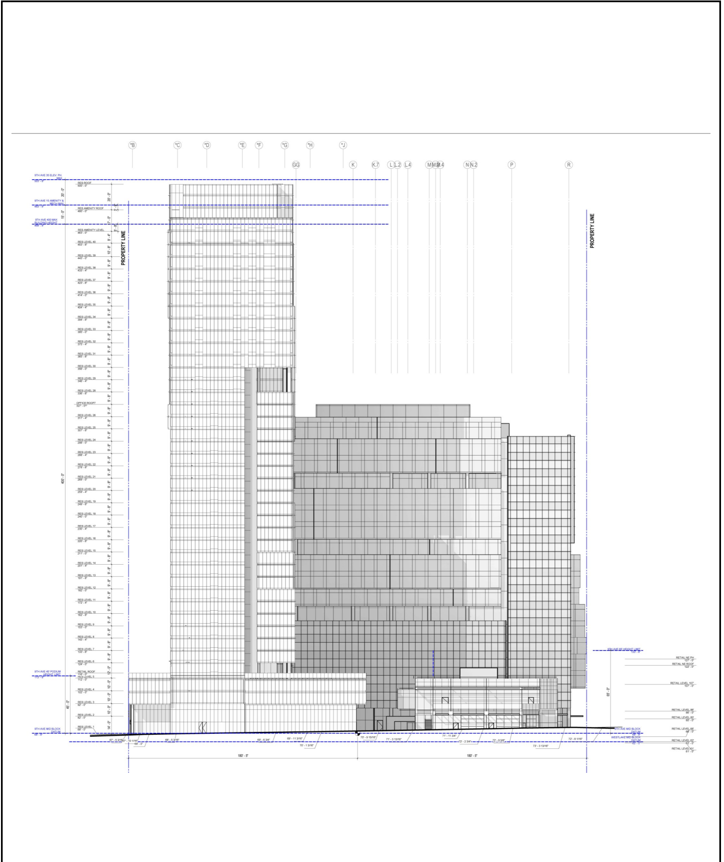
Figure 8 West Elevation
