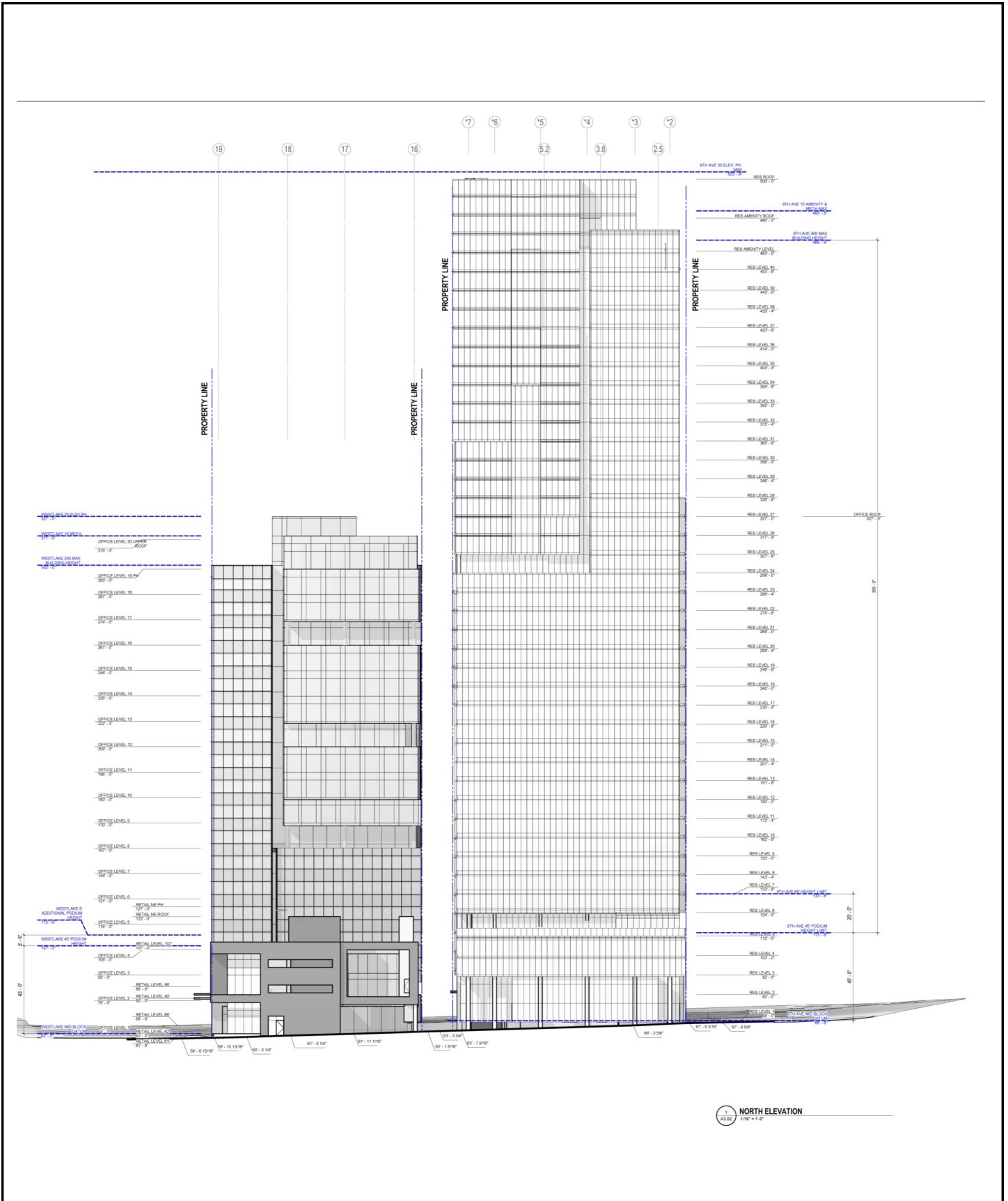
Figure 6 North Elevation
