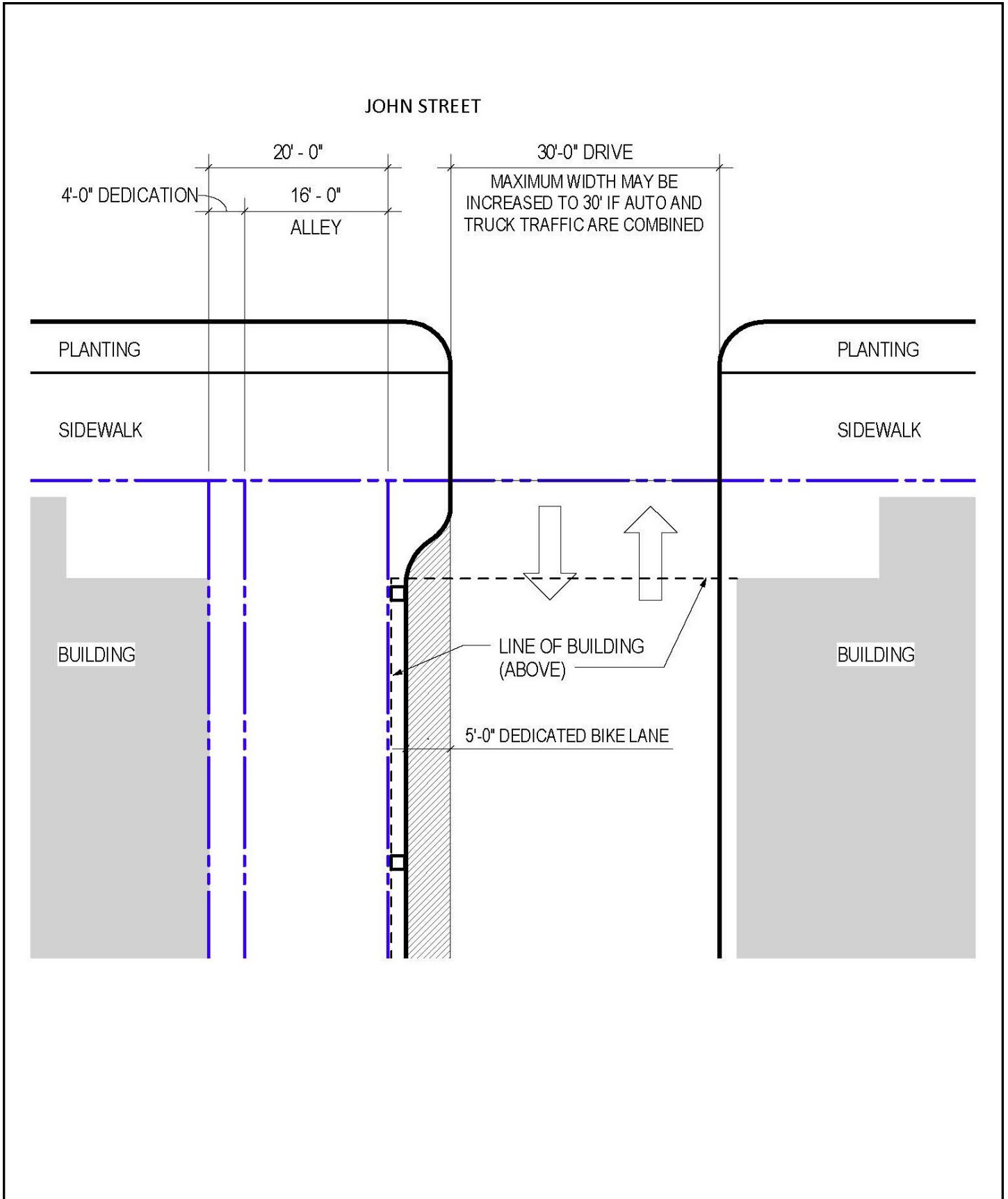
Figure 10 Site Access with Alley Vacation
