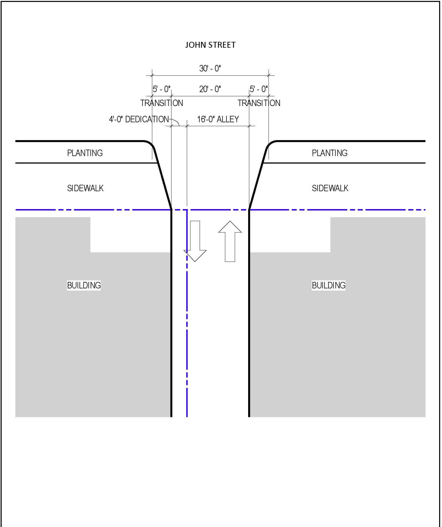
Figure 11 Site Access Without Alley Vacation
