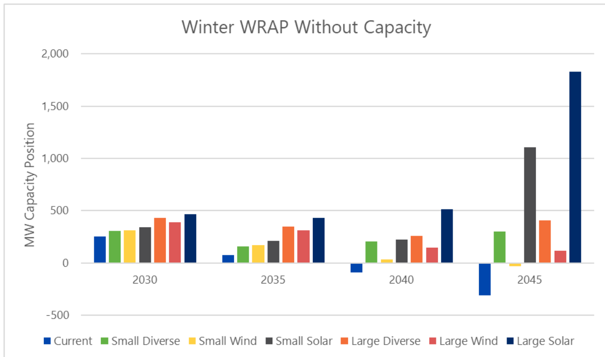
Figure 10.5. IRP 2026 Seven Portfolios Winter Greatest Monthly Deficit/Smallest Surplus Without Firm Capacity Additions
