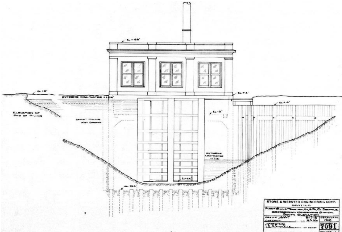
Georgetown Steam Plant Pump House, 7551 8 th Avenue S, 1915 drawing
