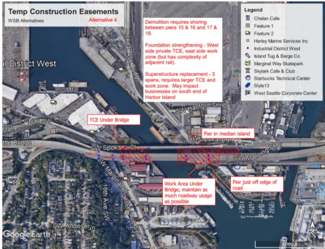
Figure 29. Temporary construction easements that would be required for Alternative 4
